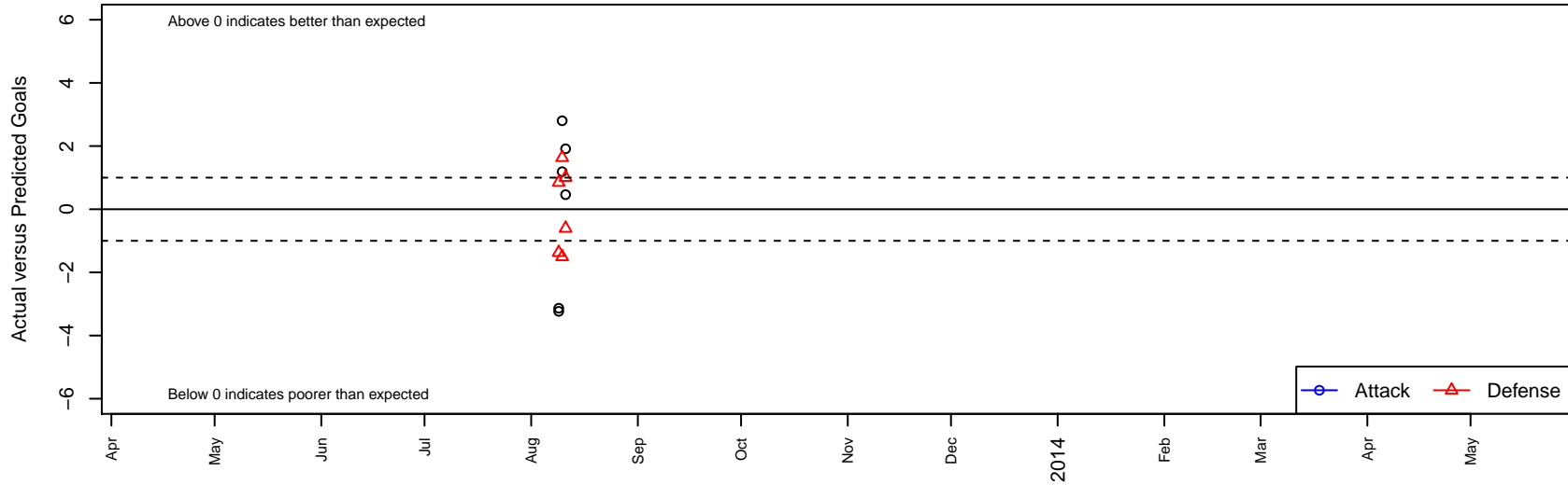
El Camino Real Salinas Galaxy B01 Dots are actual minus expected GF (blue circles) and GA (red triangles). Blue line is smoothed change in attack strength. Red is smoothed change in defense strength.
